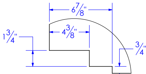
DETAIL B SCALE 1 : 6
